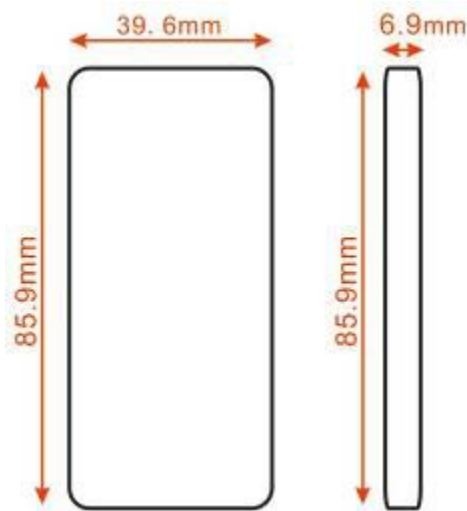
Remoter dimension
