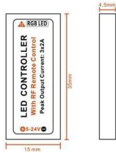
Controller dimension
